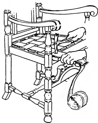
FIG. 473. PLACING THE WEBBING.
